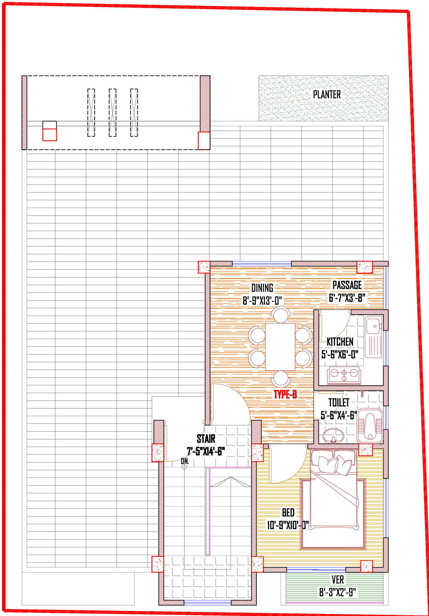
ROOF FLOOR PLAN.
